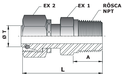
Adaptador Macho NPT Ex. AMWS 12.7x1/2 NPT.
