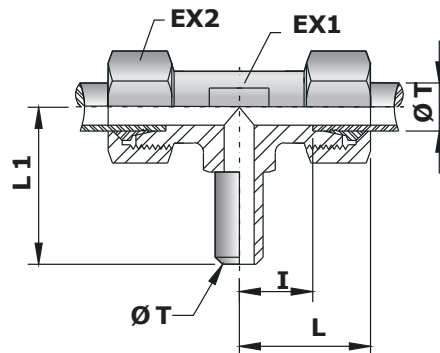
TE Ponta Lisa Ex. TLS 12.7
