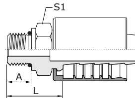
Macho Fixo UN/UNF (Male SAE Straight Thread with O-Ring - Rigid)
